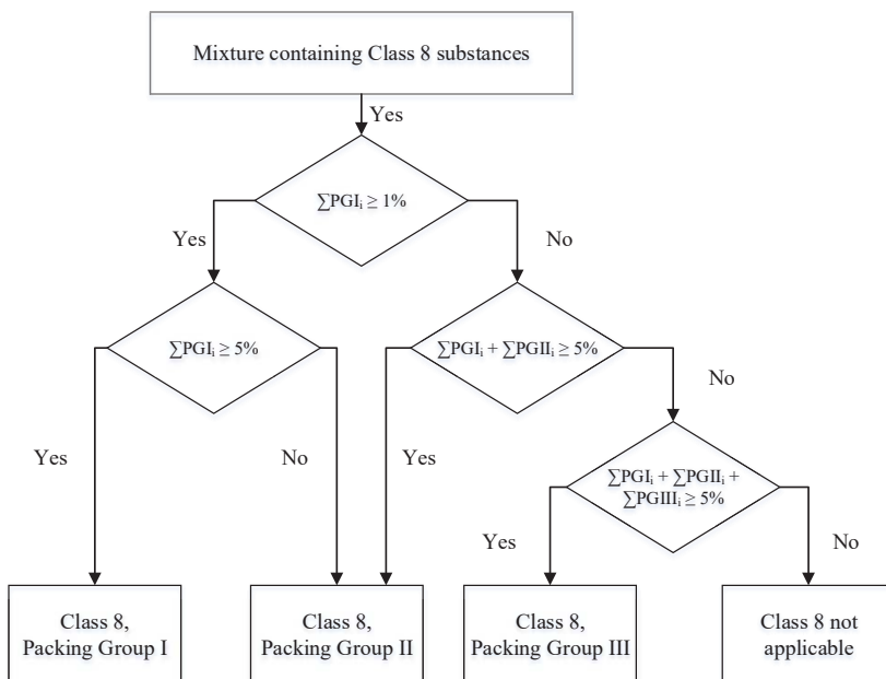
Figure 2.8.4.3: Calculation method
